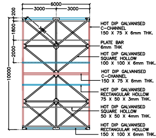
STRUCTURE LAYOUT PERMATAGRATE FRP FLOATING JETTY SCALE : 1:100
